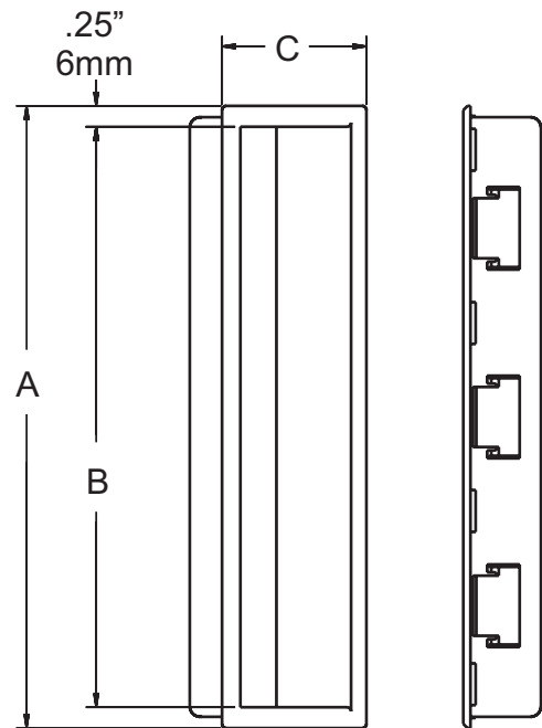
KASON 905 SERIES RECESS SNAP IN HANDLES MEASUREMENTS
